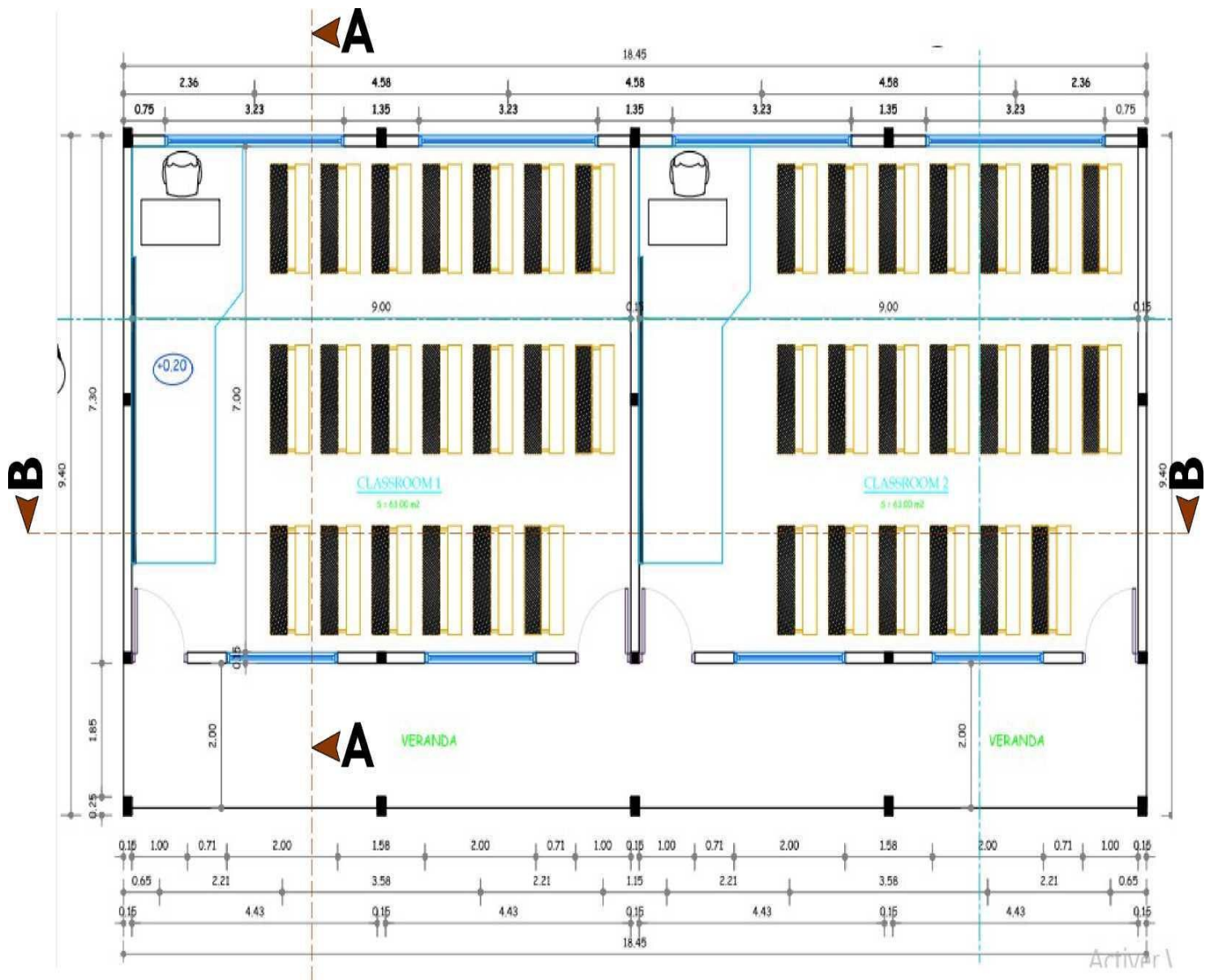
PLAN DE DISTRIBUTION - DISTRIBUTION PLAN
